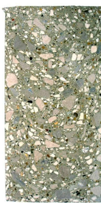
Figure 4. HVSI = 1, stable
