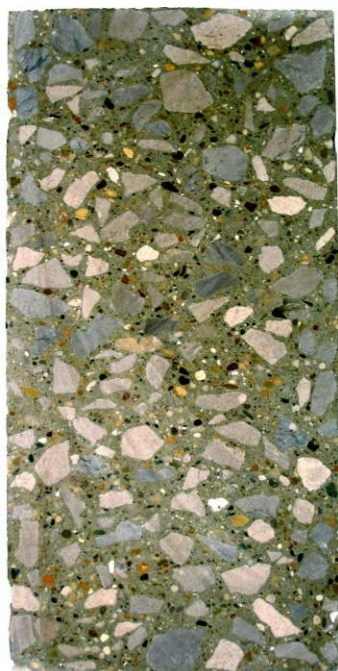
Figure 1. HVSI = 0, stable
