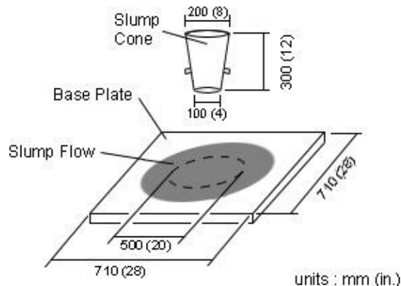
Figure 1. Slump Flow Test
