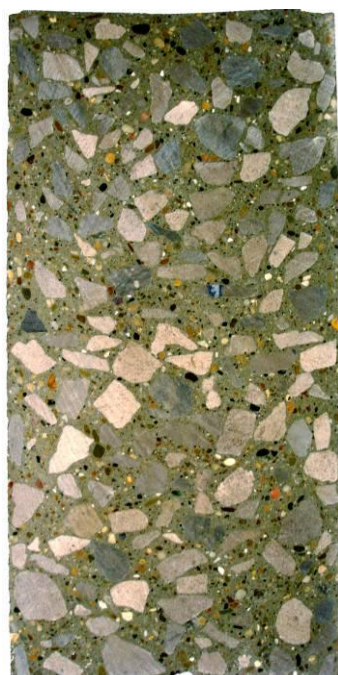
Figure 3. HVSI = 1, stable
