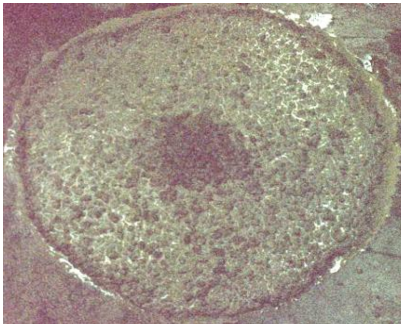
Figure 9. VSI = 3, unstable
